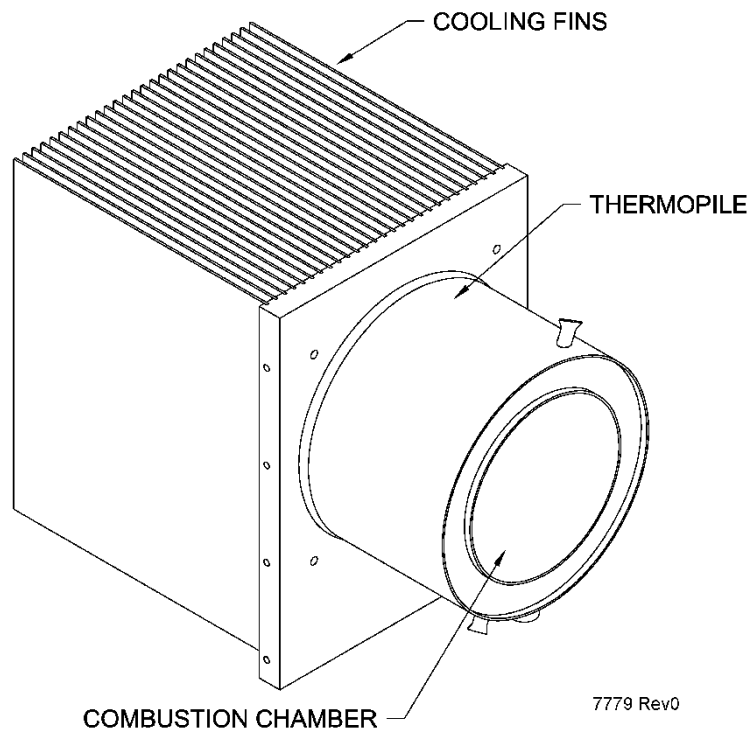
Figure 16 Power Unit
