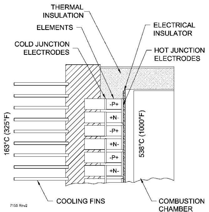
Figure 1 TEG Design
