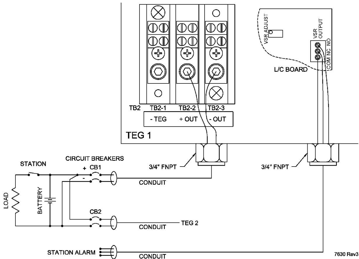
Figure 7 Recommended Connections
