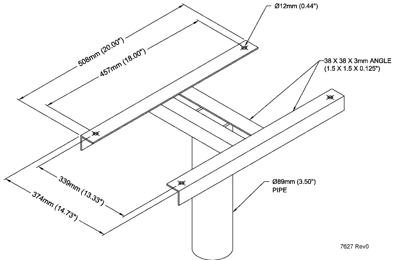
Figure 5 TEG Mounting
